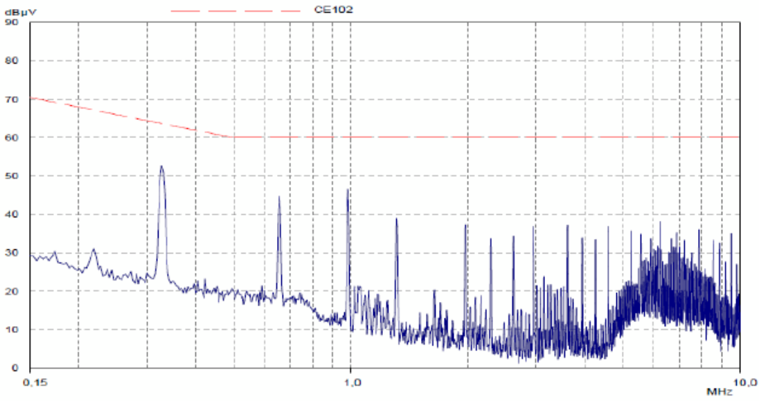
MIL-STD-461E : MGDS-15x-H-J with FGDS-10A-50V
