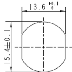
C1 Recommended Panel Cut-Out
