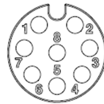
C1 Pin Assignments Front View
