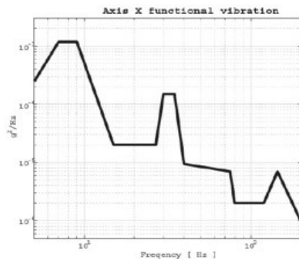
Figure 9: Axis X Tactical Functional Vibration
